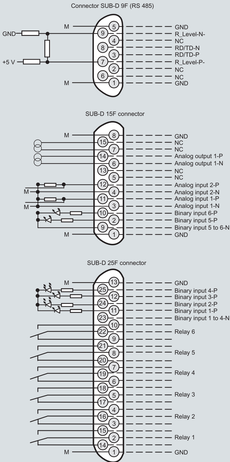
OXYMAT 6, 19" unit, pin assignment
