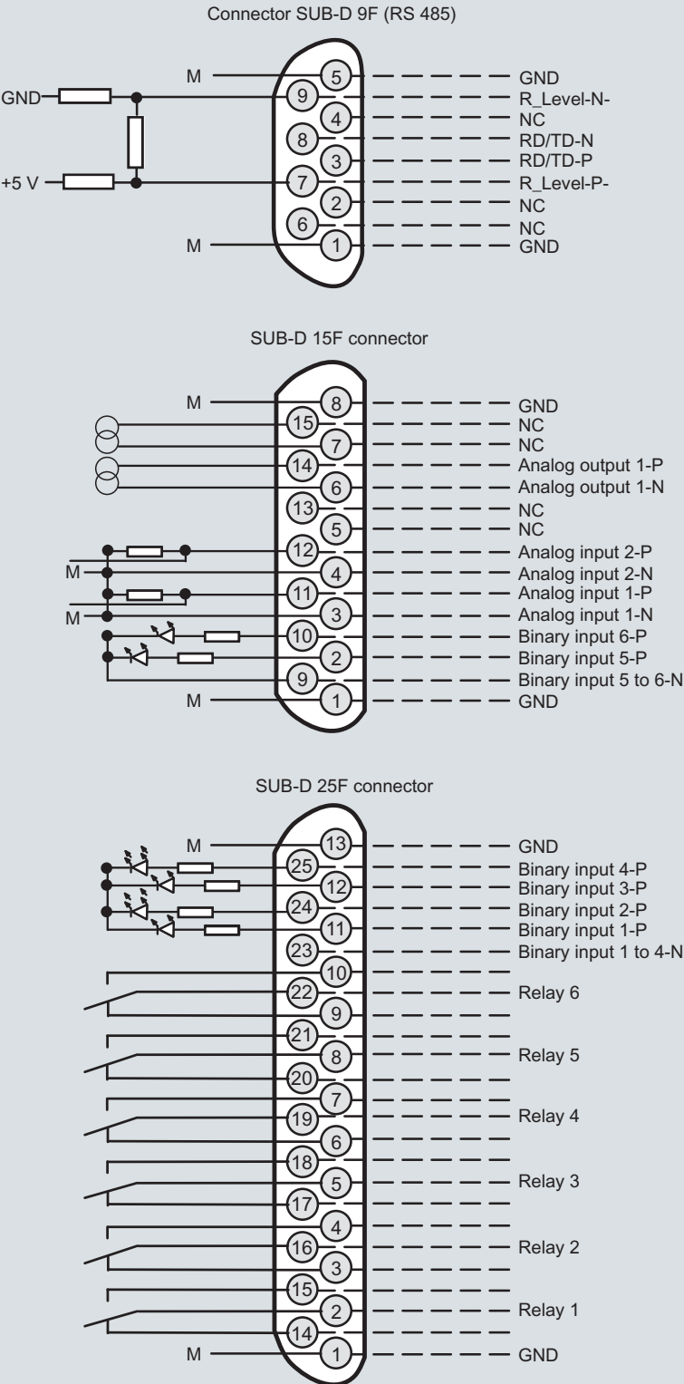
CALOMAT 6, 19" unit, pin assignment
